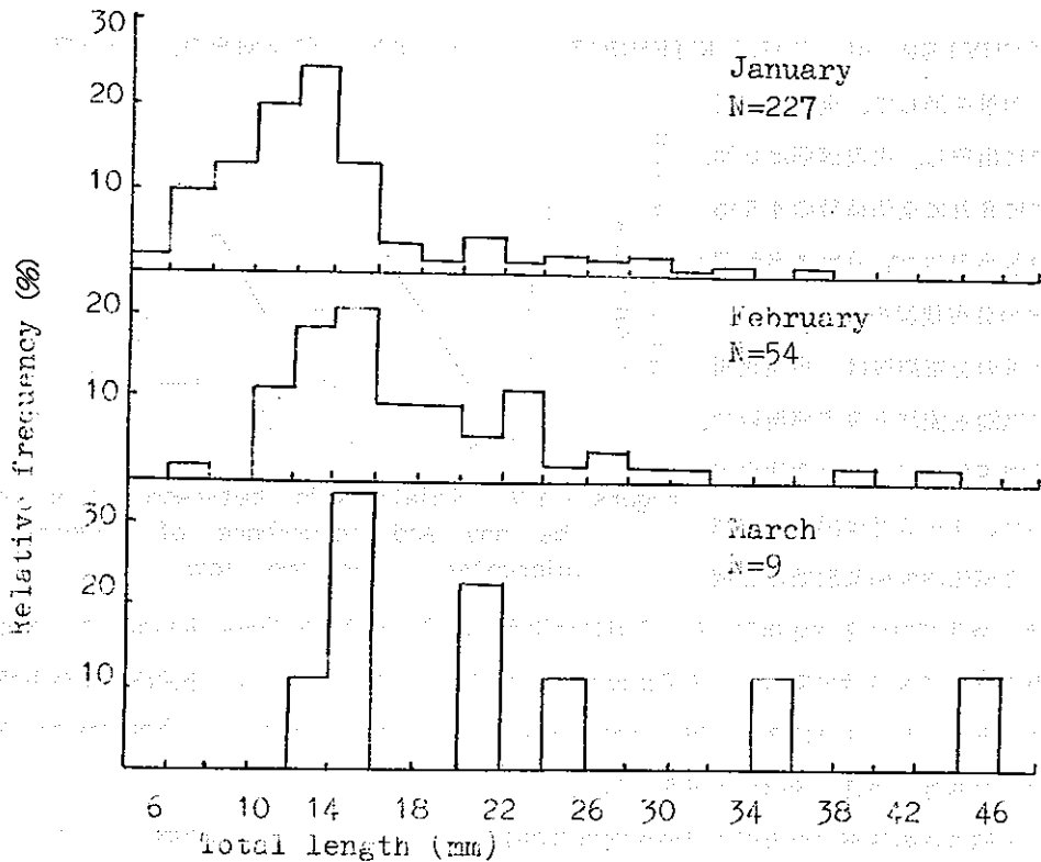
Figure-15 Monthly total length composition of larvae of Cololabis saira
