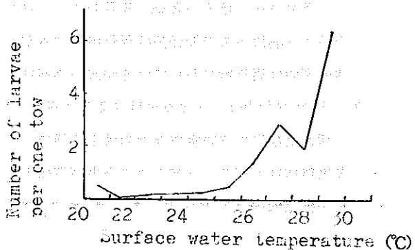
Figure-16 Relationship between surface water temperature and occurrence of Oxyporhamphus micropterus per one tow
