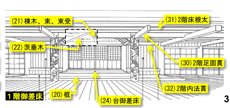
(21) 棟木、束、束受
